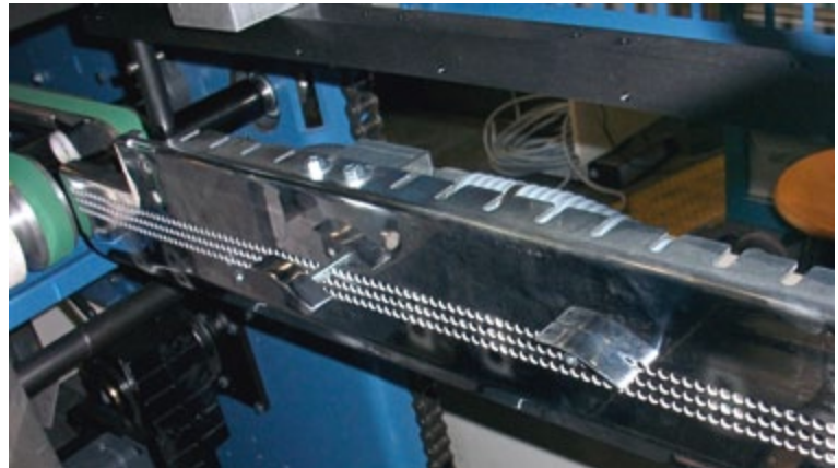
Separator finger for scroll sheets
