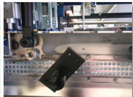
Side view with freely positionable magnets
